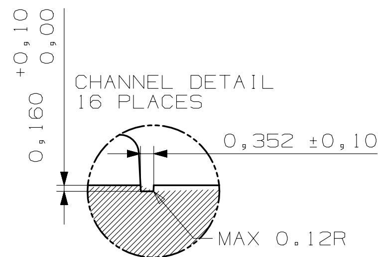
DETAIL G SCALE 10:1
